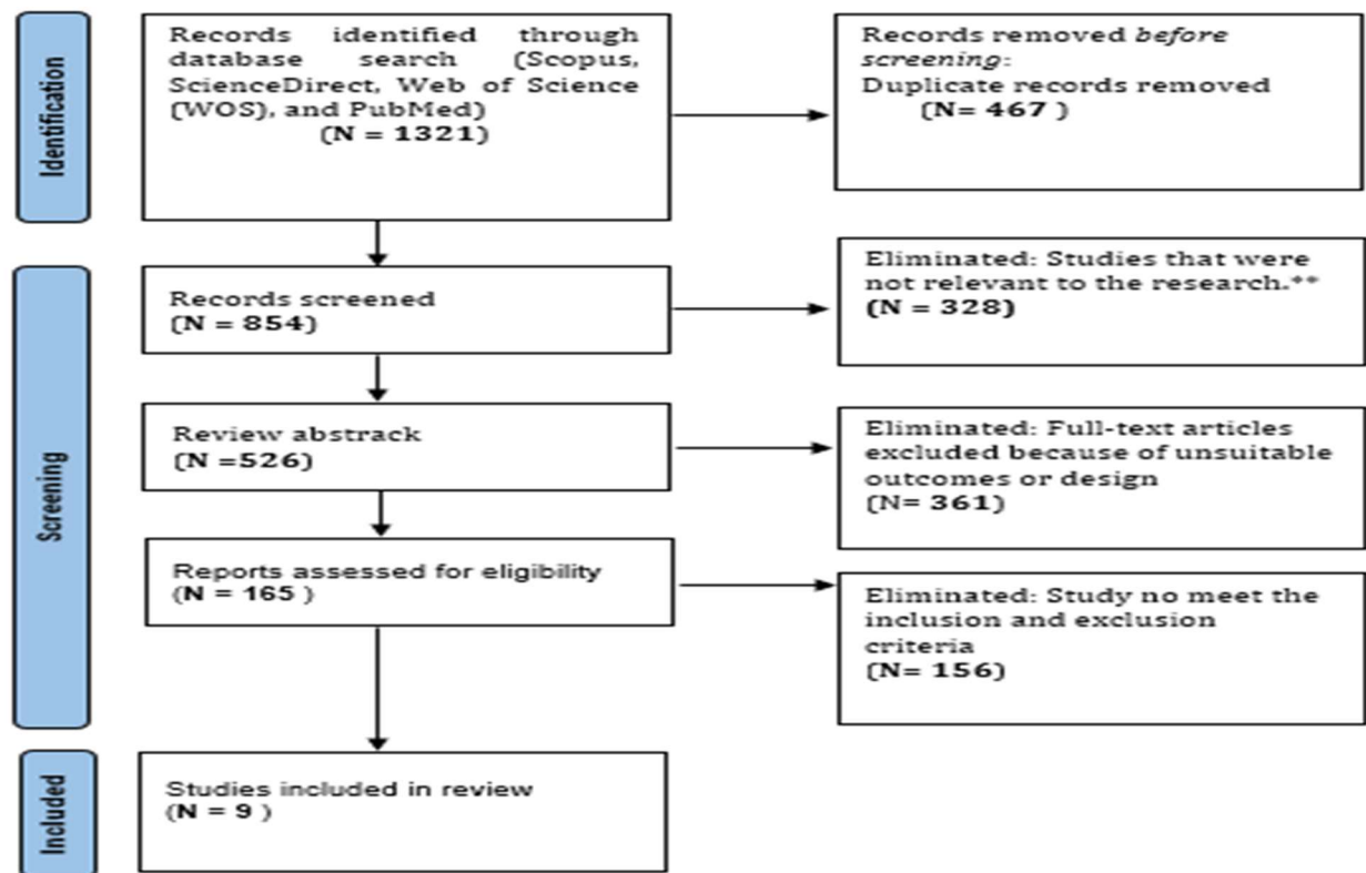
Figure 1. PRISMA Research Flowchart
